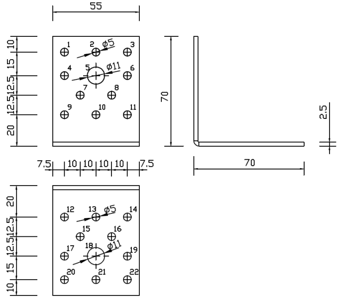
Figure A.2 Dimensions of Angle Bracket 70 without rib
